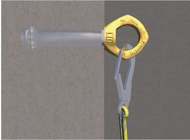
HALFEN PSA Attachment in application: DEMU T-FIXX® Fixing anchor cast in concrete with reusable eyebolt for reliable fixing of personal fall protection equipment
