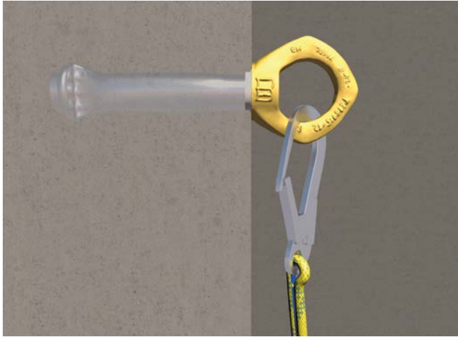
HALFEN PSA Attachment in application: HALFEN DEMU T-FIXX® Fixing anchor cast in concrete with reusable eyebolt for reliable fixing of personal fall protection equipment
