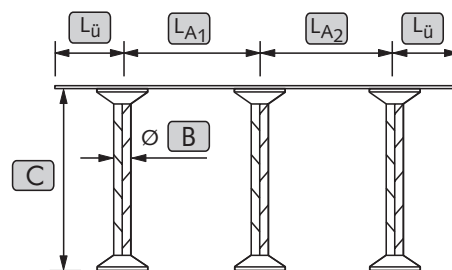
HDB-N - 3-deuvel element
